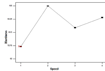
Figure.8. Hardness Vs Speed
