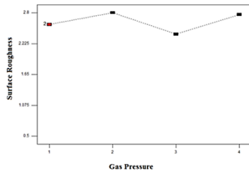
Figure.5. Surface Roughness Vs Gas Pressure
