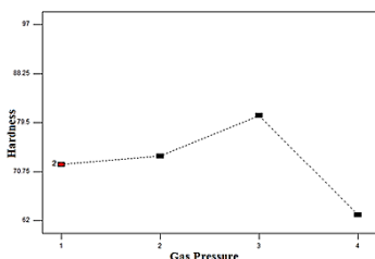
Figure.9. Hardness Vs Gas Pressure
