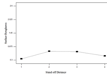
Figure.6. Surface Roughness Vs SOD
