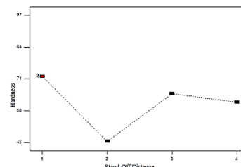
Figure.10. Hardness Vs Stand Off Distance
