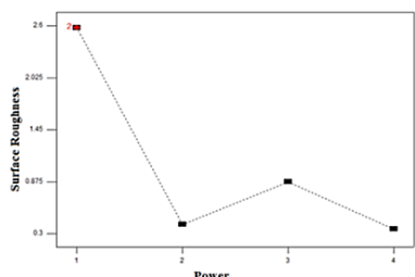
Figure.3. Surface Roughness Vs Power
